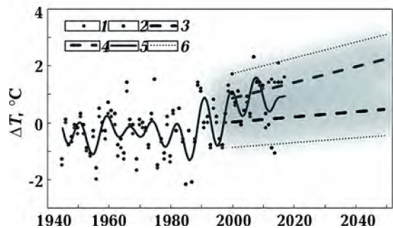
Fig. 7. Scenarios of temperature changes for the climatic landscape zone of the Northwest Greater Black Sea area (in the middle lower part of the basin of the South Bug River) by 2050: 1 — temperature anomalies of meteostation Pervomaisk, 2 — temperature anomalies of meteostations Vosnovensk, 3 — semi-empirical oscillation model, 4 — optimistic scenario, 5 — pessimistic scenario, 6 — confidence interval.
