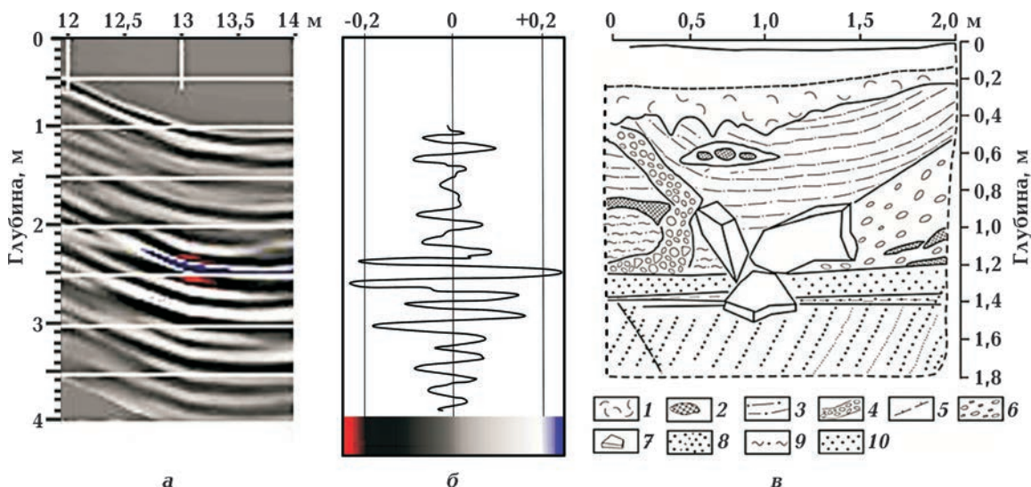
Fig. 4. Comparison of the results of georadar and geological surveys along the western wall of the pit: a — fragment of the radarogram; b — wave pattern along the route for a picket 13 m; v — a diagram of the geological structure of the western side of the exploration pit. 1 — weakly humified mass with interlayers of gravel; 2 — poorly cemented marly siltstone with cuprous concretions; 3 — silty-fine gravel; 4 — sand and gravel mixture; 5 — contours of archaeological clean-ups; 6 — gravel-pebble mixture of different types of rocks; 7 — slabs of dense arkose sandstone; 8–10 — fine-grained sandstone.
