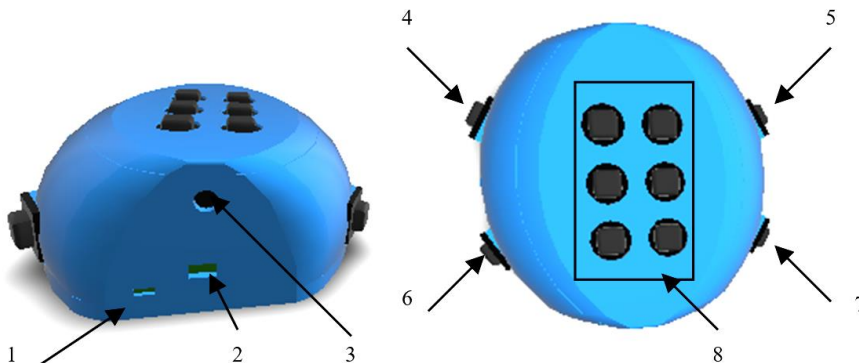
Fig. 1. Components of the hardware and software complex of Braille training: 1 – power button; 2 – miniUSB connector; 3 – power connector; 4 – input button; 5 – cancel button; 6 – left navigation button; 7 – right navigation button; 8 – six letter buttons in Braille
