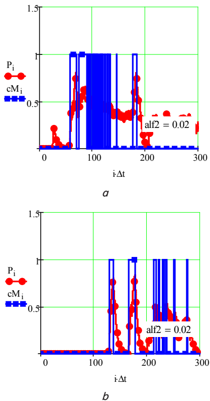
Fig. 6. Results of verification of FD self-adjusting by smoke density, at fixed parameter g[\gamma]=0.05 : a – alcohol; b – wood
