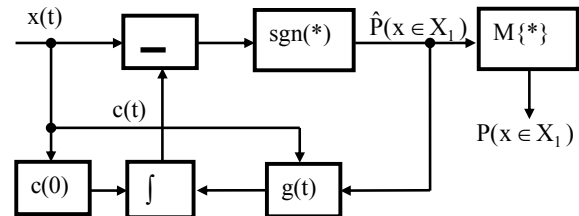
Fig. 2. Block diagram of FD capable of self-learning by ignition of materials for guaranteed detection of fire source at sites
