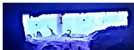
Fig. 12. Experimental lance (varied nozzle inclination angles): 1 – lance; 2 – CO bubble (when blowing the bath ([C]=2.5 % with an oxygen flow rate through the lance of 2,000 m 3 /h)
