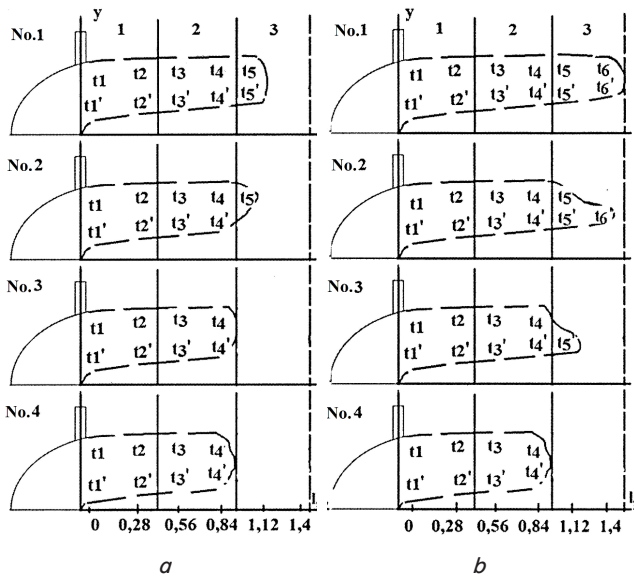
Fig. 6. Schematic representation of contours of the visible part of temperature fields of the drifted flame on the basic (a) and experimental (b) lances based on the results of measurements in TSU at different intensities of blowing the bath with oxygen: 1, 2, 3 – zones of the flame, t 1 – t 6 – points of temperature measurements of the top part of the flame, °C; t 1 '– t 6 ' – points of temperature measurements of the bottom part of the flame, °C; l z – flame length, m
