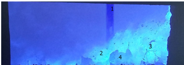
Fig. 3. Image of the near-lance flame formed when blowing the bath ([C]=3 %) with an oxygen flow rate through the lance of 2000 m 3 /h: 1 – lance; 2 – flame; 3 – metal splashes; 4 – CO bubble at tearing of the oxide film
