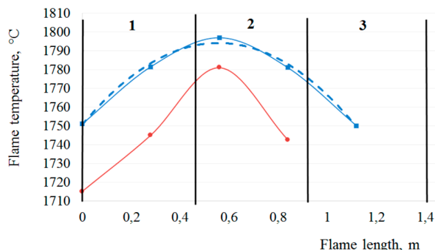
Fig. 9. Distribution of temperature fields of the drifted flame when using experimental and basic lances with a carbon content of 3 %; dotted line marks estimated dependence for experimental lance with the intensity of blowing the melt with oxygen at 2,000 m 3 /h (experiment No. 3): — experimental lance; — basic lance; - - - polynomial (experimental lance)
