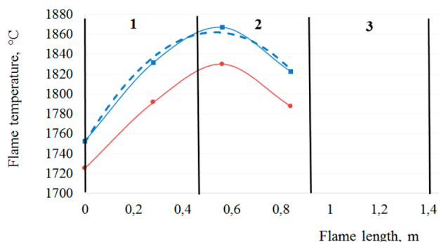
Fig. 10. Distribution of temperature fields of the drifted flame when using experimental and basic lances with a carbon content of 3 %; dotted line marks estimated dependence for experimental lance with the intensity of blowing the melt with oxygen at 1,800 m 3 /h (experiment No. 4): — experimental lance; — basic lance; - - - polynomial (experimental lance)
