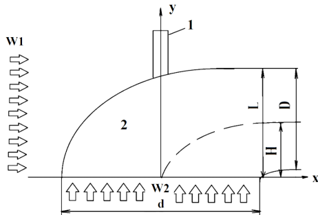
Fig. 2. Schematic of a near-lance flame formed when blowing the bath ([C]=3 %) with an oxygen flow rate through the lance of 2,000 m 3 /h: 1 – lance; 2 – flame; W1 – velocity of the entraining flue gas flow; W2 – carbon monoxide flow velocity
