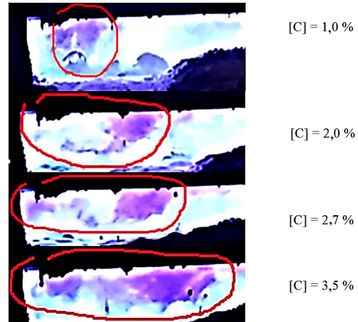
Fig. 4. Formation of the flame lengthwise the bath, drifted by the flow of flue gases at a different content of carbon in the melt
