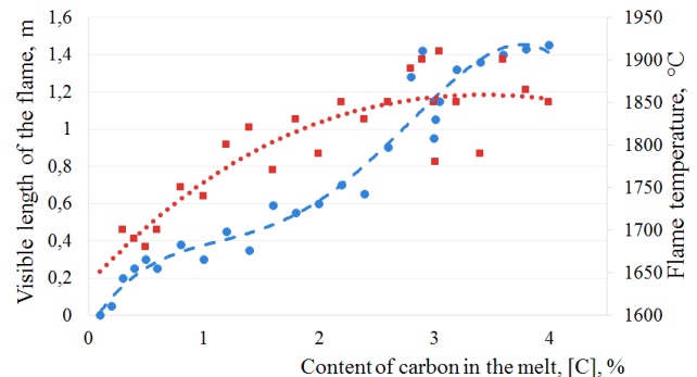
Fig. 5. Change in the length and temperature of the drifted flame on TSU at a different content of carbon in the melt (at intensity of oxygen blowing 2,200 m 3 /h):
