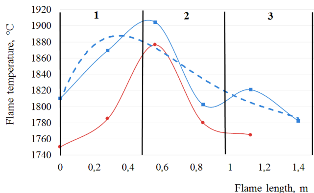
Fig. 7. Distribution of temperature fields of the drifted flame when using experimental and basic lances with a carbon content of 3 %; blowing intensity 2,400 m 3 /h (experiment No. 1): —■— experimental lance; —●— basic lance; - - - polynomial (experimental lance)
