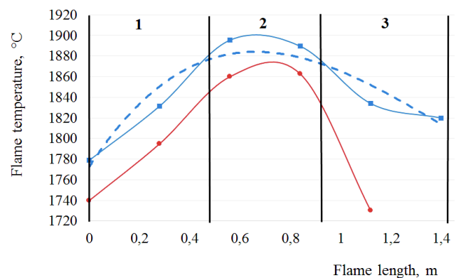
Fig. 8. Distribution of temperature fields of the drifted flame when using experimental and basic lances with a carbon content of 3 %; blowing intensity 2,200 m 3 /h (experiment No. 2): —■— experimental lance; —●— basic lance; - - - polynomial (experimental lance)
