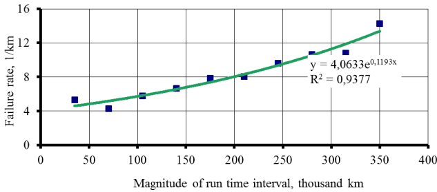
Fig. 4. Chart of failure rate \lambda(l) of traction electric motors in dependence on the run time interval \Delta l
