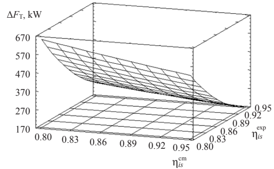
Fig. 5. Influence of \eta_{is}^{exp} and \eta_{is}^{cm} on \Delta F_T
