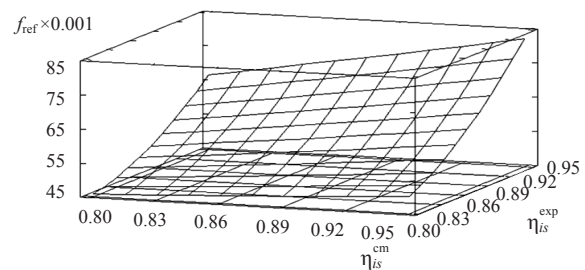
Fig. 8. Influence of \eta_{is}^{exp} and \eta_{is}^{cm} on f_{ref}
