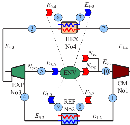
Fig. 1. Scheme of decomposition of exergy flows in the ARM
