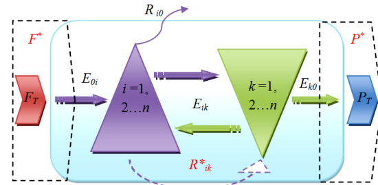
Fig. 2. A generalized diagram of the image of the target exergy flows in the installation
