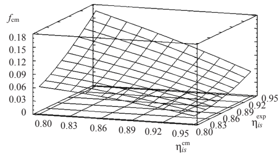
Fig. 7. Influence of \eta_{is}^{exp} and \eta_{is}^{cm} on f_{cm}
