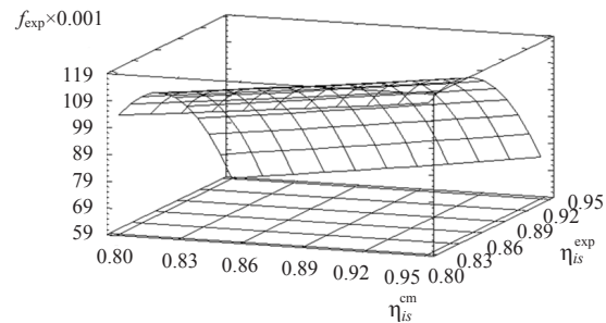
Fig. 6. Influence of \eta_{is}^{cm} and \eta_{is}^{exp} on f_{exp}
