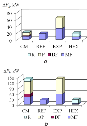
Fig. 4. The nature of distribution of exergy losses in the ARM elements when the isentropic efficiency of the compressor and the turboexpander vary: \eta_{is}^{cm} = 0.95 , \eta_{is}^{exp} = 0.875 (a); \eta_{is}^{cm} = 0.8 , \eta_{is}^{exp} = 0.8 (b)
