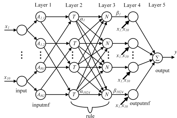
Fig. 3. The structure of the neural-fuzzy ANFIS network
