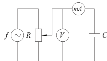
Fig. 1. Measuring method of dielectric permittivity of oil by using voltmeter-ammeter
