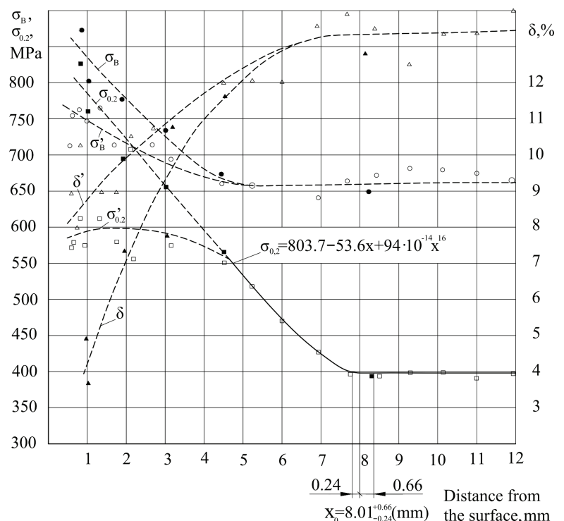
Fig. 1. Mechanical properties of the surface layer of the shafts reeled with toroidal rollers with diameter D_p = 105 mm, profile radius r_p = 10 mm: \sigma_B , \sigma_{0.2} and \delta are properties in a circular direction; \sigma'_B , \sigma'_{0.2} , \delta' are properties in the axial direction
