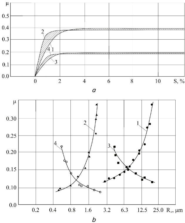
Fig. 4. Dependence of the coefficient of friction: on the magnitude of slip (a); on the surface roughness (b): non-reeled nonlubricated specimen (1); the nonlubricated specimen reeled with a roller (2); the non-reeled lubricated specimen (3); the lubricated specimen reeled with a roller (4)
