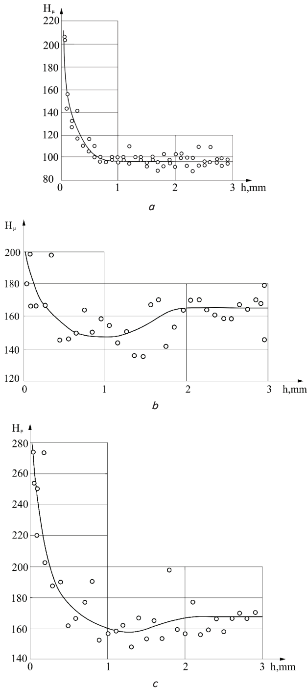
Fig. 3. Distribution of microhardness in the depth of the hardened layer: Armco iron, r_p=2.5 mm, P=1.5 kN (a); 45 grade steel, r_p=5 mm, P=5 kN (b); 40X grade steel, r_p=2.5 mm, P=5.5 kN (c)
