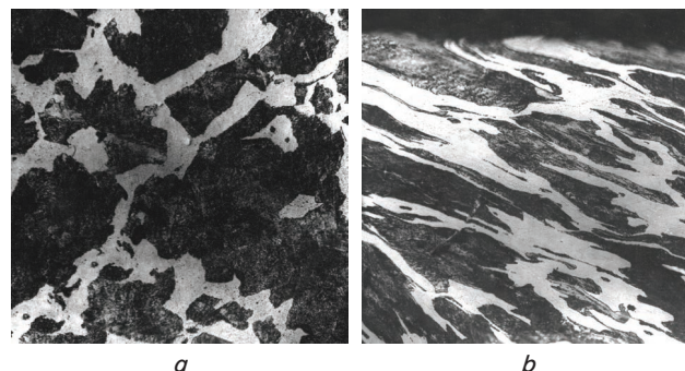
Fig. 2. Microstructure of specimens of the surface layer of normalized 40 grade steel: before reeling ( a ); after reeling ( b ) ( \times 300 )
