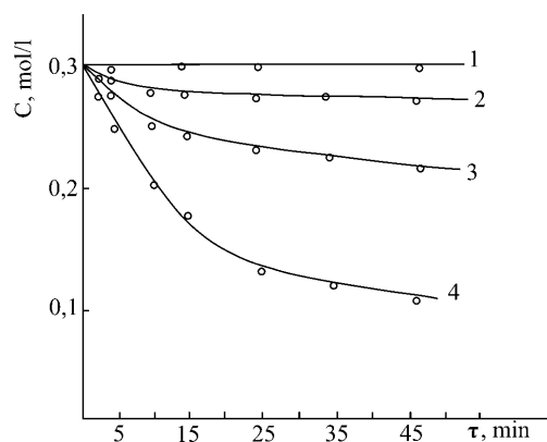
Fig. 6. Kinetic curves of thermal decomposition of ozonides of 4-bromethylbenzene at 20 (1); 30 (2); 40 (3); 50 °C (4)
