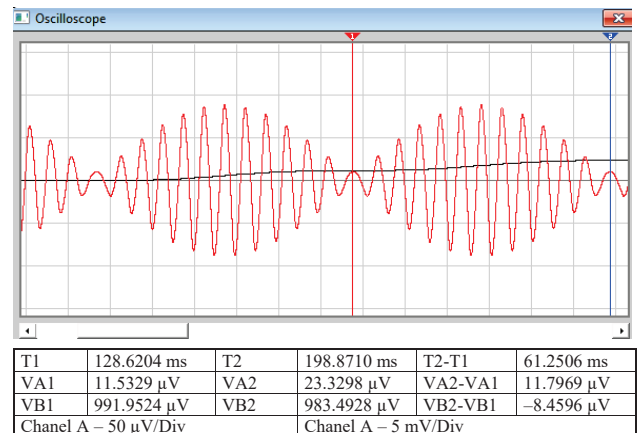
Fig. 5. Time diagram of the signal of damage to an inner ring
