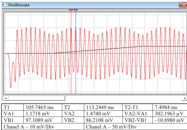
Fig. 3. Time diagram of the signal of damage to rolling bodies
