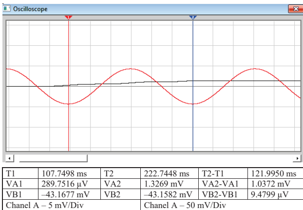
Fig. 4. Time diagram of the signal of damage to an outer ring
