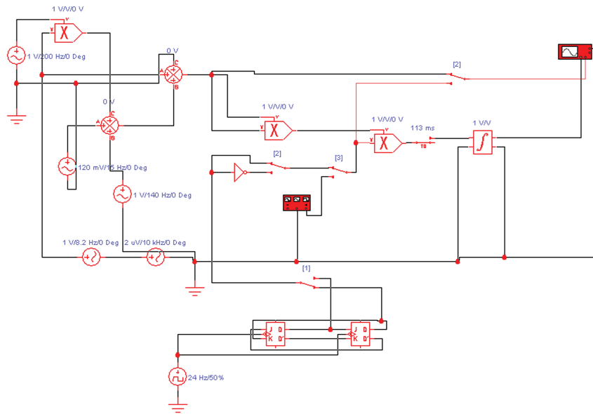
Fig. 6. Diagram of RMS detector with a model of the filter's output signal at actual input signals
