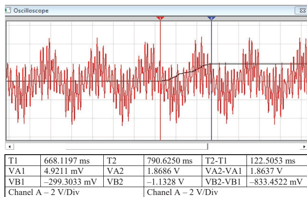
Fig. 7. Result of measuring a signal at the output of RMS detector
