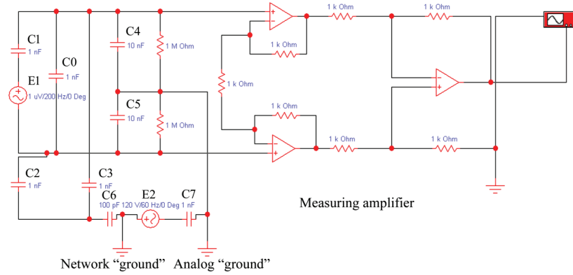
Fig. 8. Model of electrometric measuring amplifier with differential-current inputs for operation with piezoelectric sensors
