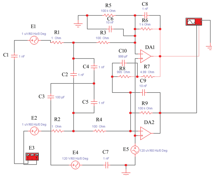
Fig. 9. Model of charge measuring amplifier with differential-current inputs for operation with piezoelectric sensors
