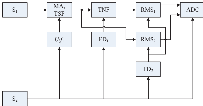
Fig. 1. Device for vibration diagnosis of bearing assemblies
