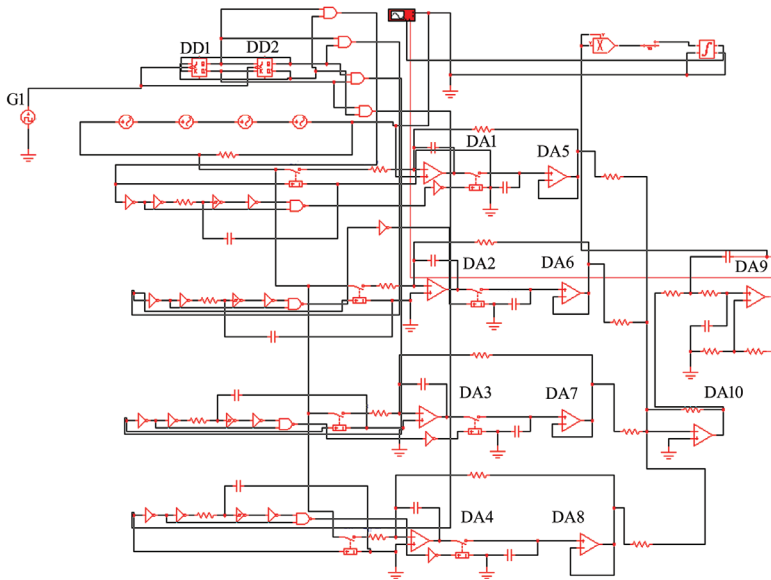
Fig. 2. Diagram of the 4-channel filter with a coefficient of window overlap k=1
