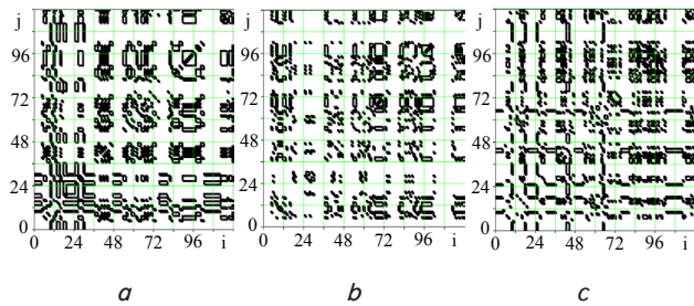
Fig. 2. Recurrent plots (2) for NO 2 concentrations in the atmospheric air of the typical urban configuration at control points: a – A; b – B; c – C
