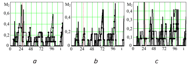
Fig. 4. Dynamics of measure M_2 of RS for NO 2 concentration in the atmospheric air at control places: a – A; b – B; c – C
