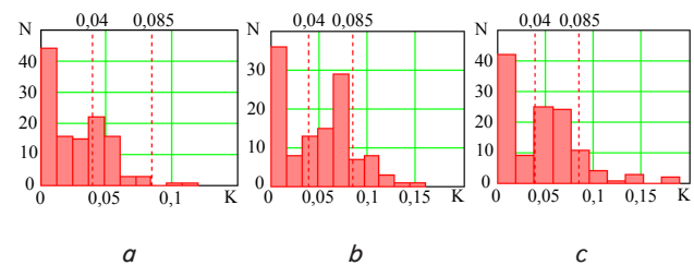
Fig. 5. Histograms of NO 2 concentrations in the atmospheric air for control points: a – A; b – B; c – C
