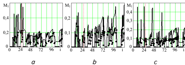
Fig. 3. Dynamics of measure M_1 of RS for NO 2 concentration in the atmospheric air at control places: a – A; b – B; c – C
