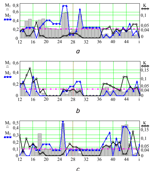
Fig. 6. Comparative dynamics of measures M_1 and M_2 of RS for NO 2 concentration in the atmospheric air, as well as dynamics of the measured NO 2 concentration and magnitude of MAC for assigned control points: a – A; b – B; c – C
