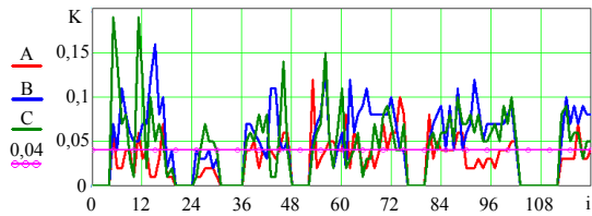
Fig. 1. Values of measured concentration (mg/m 3 ) of NO 2 in atmospheric air of the typical urban configuration at controls points A, B, C
