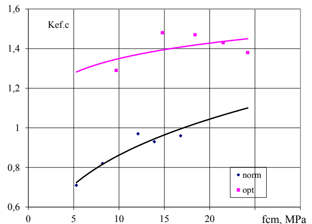
Fig. 2. Dependence of cement utilization factor on concrete strength
