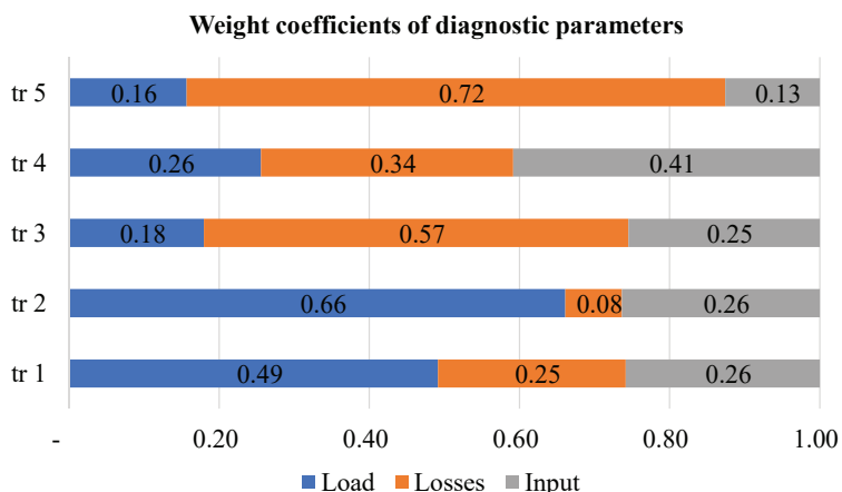
Fig. 2. Weight coefficients of diagnostic parameters
