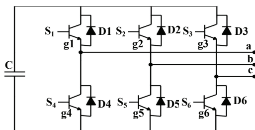
Fig. 2. Three phase VSC
