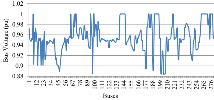
Fig. 5. Voltage profile of KR power system without STATCOM
