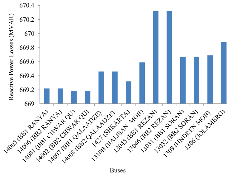
Fig. 8. Reactive power losses with STATCOM of optimal size at different weak buses
