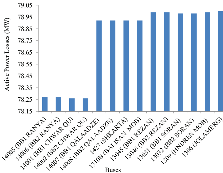
Fig. 7. Active power losses with STATCOM of optimal size at different weak buses
