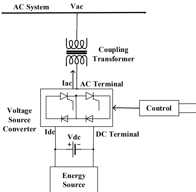
Fig. 1. Basic components of STATCOM
