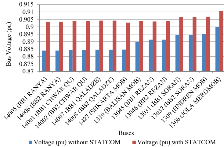
Fig. 6. Low voltage buses before and after STATCOM Connection
