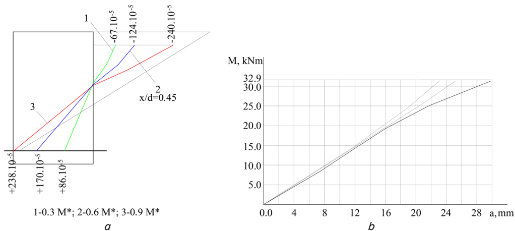
Fig. 9. Diagram of beam destruction: a – distribution of strains across the cross-section height of the beam B-18-1; b – vertical deflections of the span of the beam B-18-1
