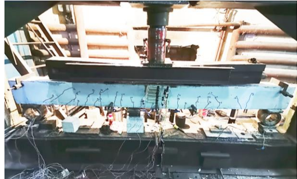
Fig. 4. General view of reinforced concrete beam tests
