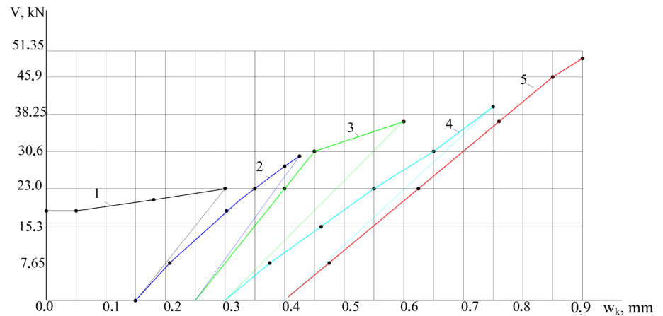
Fig. 8. Evolution plot of inclined cracks in the beam B-18-1
