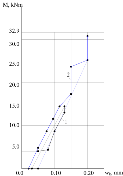
Fig. 7. Evolution plot of normal cracks in the beam B-18-1
