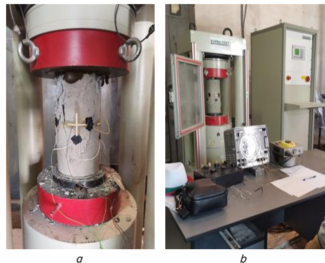
Fig. 2. Concrete cylinder: a – test at the hydraulic press ALPHA 3-3000S; b – devices to register strains
