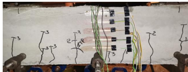
Fig. 5. General view of load cells on concrete, normal cracks, and damage area of compressed concrete zone
