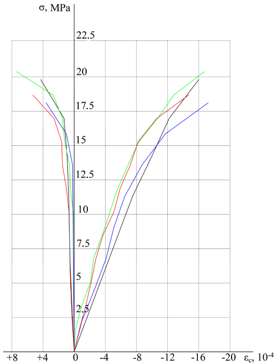
Fig. 3. Diagram of longitudinal and transverse strains of concrete cylinders
