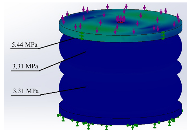
Fig. 11. Stress in the material of the flexible shell at an excess air pressure in its cavity of 1.0 MPa and with an angular displacement of the upper bottom relative to the lower one by 3.5°
