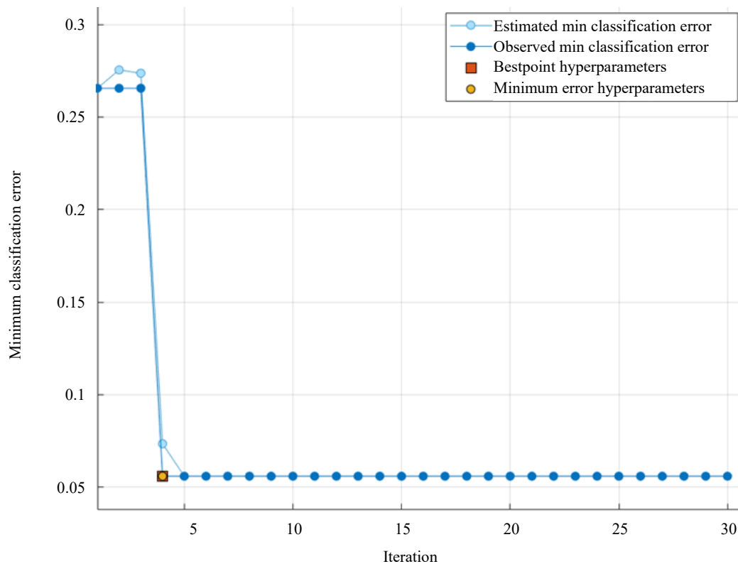
Fig. 11. The minimum classification error over 30 iterations for Optimizable KNN model
