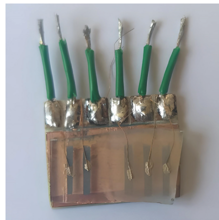
Fig. 1. General view of the resulting nanostructured sample of ZnO
