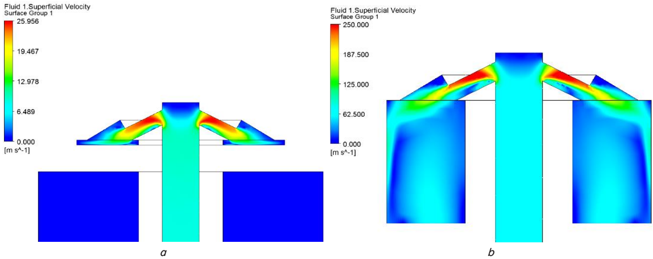
Fig. 12. Position of the bottom of the piston: a – 0.002 s after the supply of control air; b – 0.012 s after supplying control air
