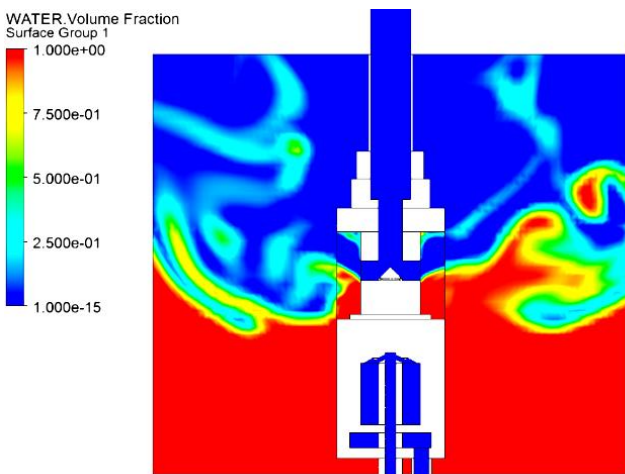
Fig. 14. Volumetric water content in the space near the valve ( t=0.06 s)
