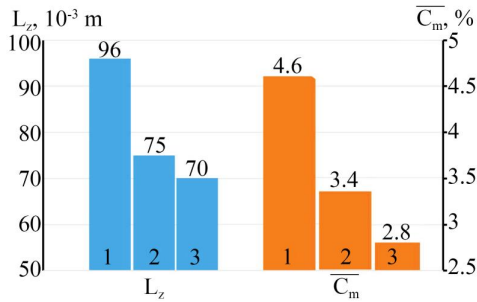
Fig. 3. The values of the inverse current zone length L_z and the average methane concentration \bar{C}_m in this zone at \alpha=1.1 ; S/d=5,6 ; d=2.5 \cdot 10^{-3} m for different rows of gas supply holes: 1, 2, 3 – number of row of holes N_R corresponding to L_1=10 \cdot 10^{-3} m; 20 \cdot 10^{-3} m, and 30 \cdot 10^{-3} m, respectively
