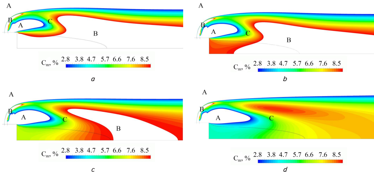
Fig. 5. Methane concentration fields in the longitudinal section of the burner module passing through the axis of the gas supply holes at \alpha=1.1 ; L_1=10 \cdot 10^{-3} m for different values of the relative pitch S/d of the location of the holes: a – S/d=4.7 ; b – S/d=5.0 ; c – S/d=5.2 ; d – S/d=5.4
