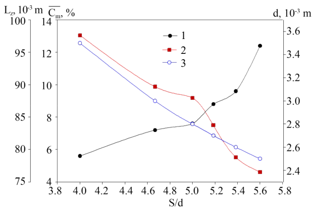
Fig. 4. Dependence of the characteristics of the reverse current zone behind the flame stabilizer and the diameter of the gas supply holes d on the relative pitch of their location at \alpha=1.1 ; L_1=10 \cdot 10^{-3} m: 1 – the length of the reverse current zone L_z ; 2 – the average value of methane concentration \bar{C}_m in this zone; 3 – the diameter of the gas supply holes
