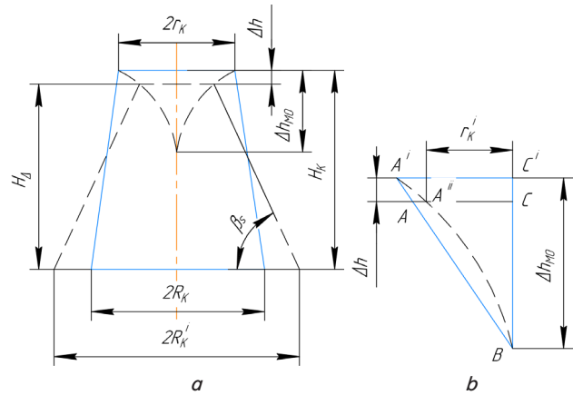
Fig. 6. The estimation scheme of changing the geometric parameters of the stack of concrete mix during settling: a – the maximum angle of the natural slope of a standard cone; b – upper radius of a standard cone
