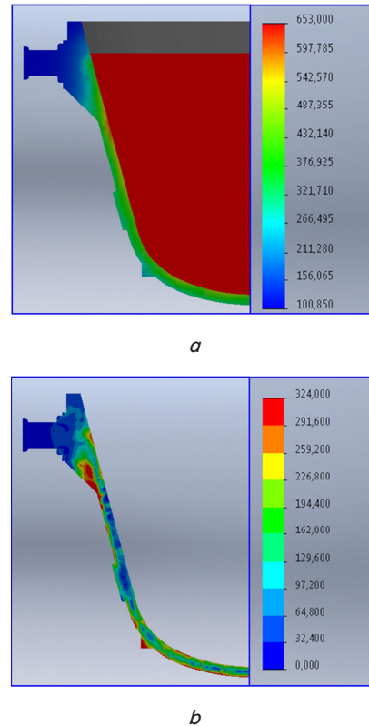
Fig. 6. Comparison of temperature fields and temperature stresses at a given level of slag for steel 30 HML: a – temperature field, °C, b – stress fields, MPa
