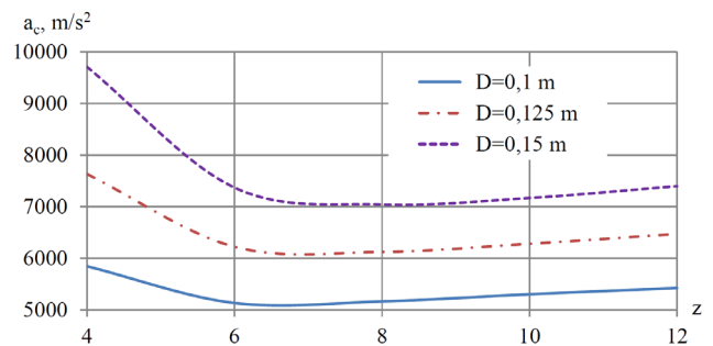
Fig. 3. Influence of amount of openings z and diameter of rotor D on the average acceleration a_c
