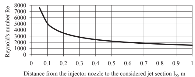
Fig. 5. The value of the Reynold's number by the jet length l_{ef} for the emulsion based on rapeseed oil at a temperature t=40\text{ }^\circ\text{C} , injector pressure P_i=0.02\text{ MPa} , injector nozzle diameter d_i=10\text{ mm}
