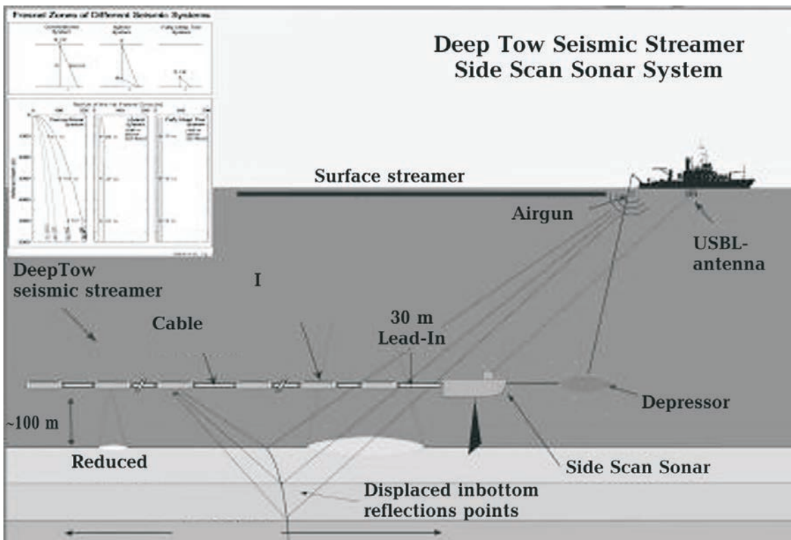
Fig. 3. The DeepTow system with multichannel streamer and Sidescan.
