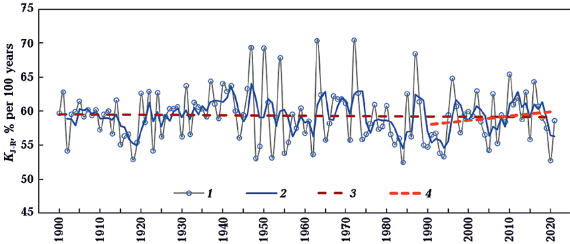
Fig. 15. Long-time changes of the thermal continentality index K_{J-R} (1) in Ukraine from 1900 to 2021 (2—sliding averaging, 3, and 4—linear trend for the period 1900—2021 and 1991 to 2020). Statistically significant trends ( \sigma < 0.05 ).
