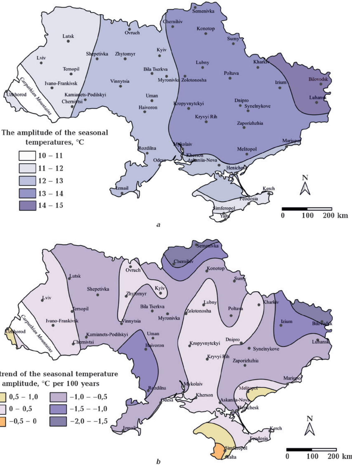
Fig. 14. The spatial distribution of the seasonal air temperature amplitude (a) and their trends (b) in Ukraine from 1900 to 2021.
