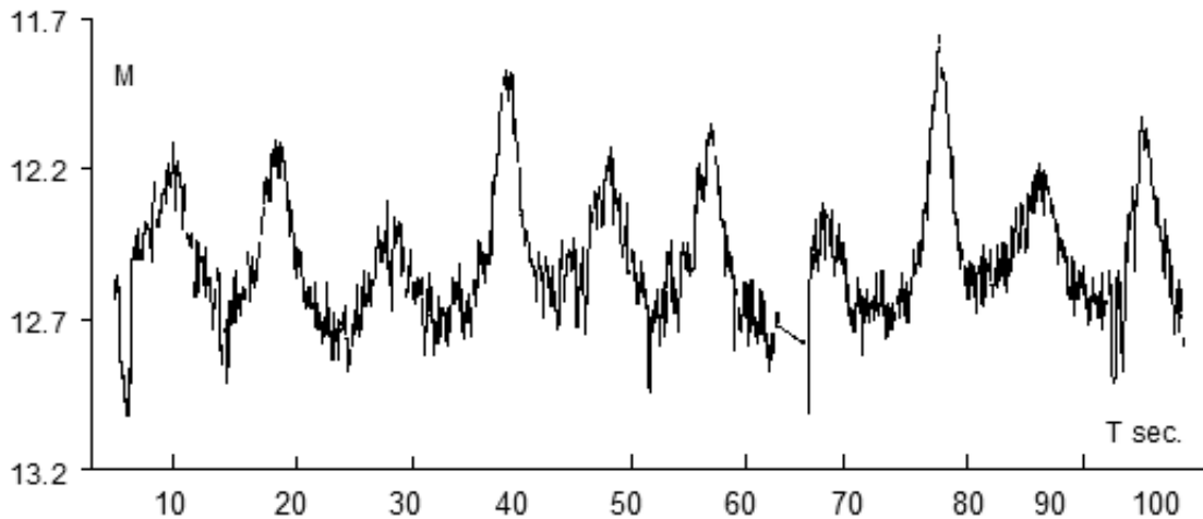
Fig.4. A fragment of the light curve of "DSP-18", V-band, 29 Sep 2014. T_{exp} = 0.2 sec.
