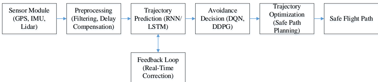
Fig. 2. Block diagram of the UAV obstacle avoidance system architecture
