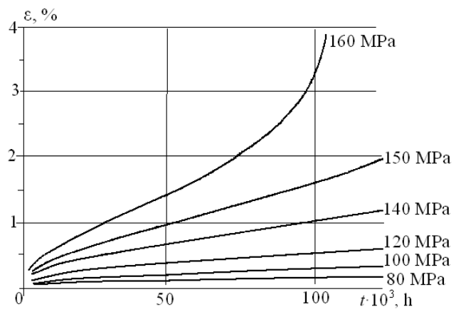
Fig. 4. Creep curves of the diaphragm material
