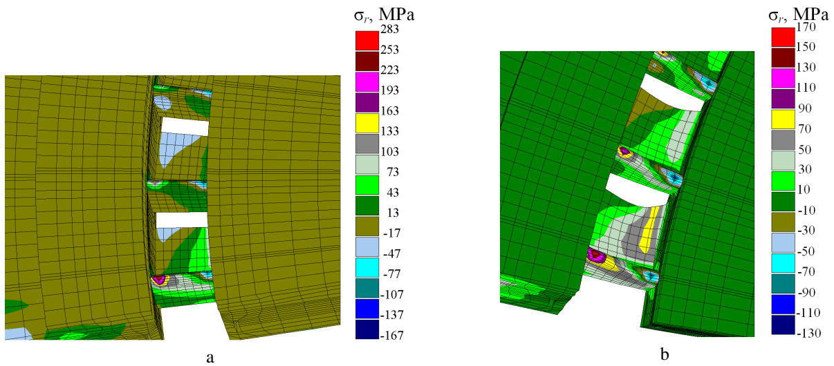
Fig. 8. Radial (along the guide vanes) stresses in the diaphragm guide vanes near the joint face: a – in the elastic state; b – during creep
