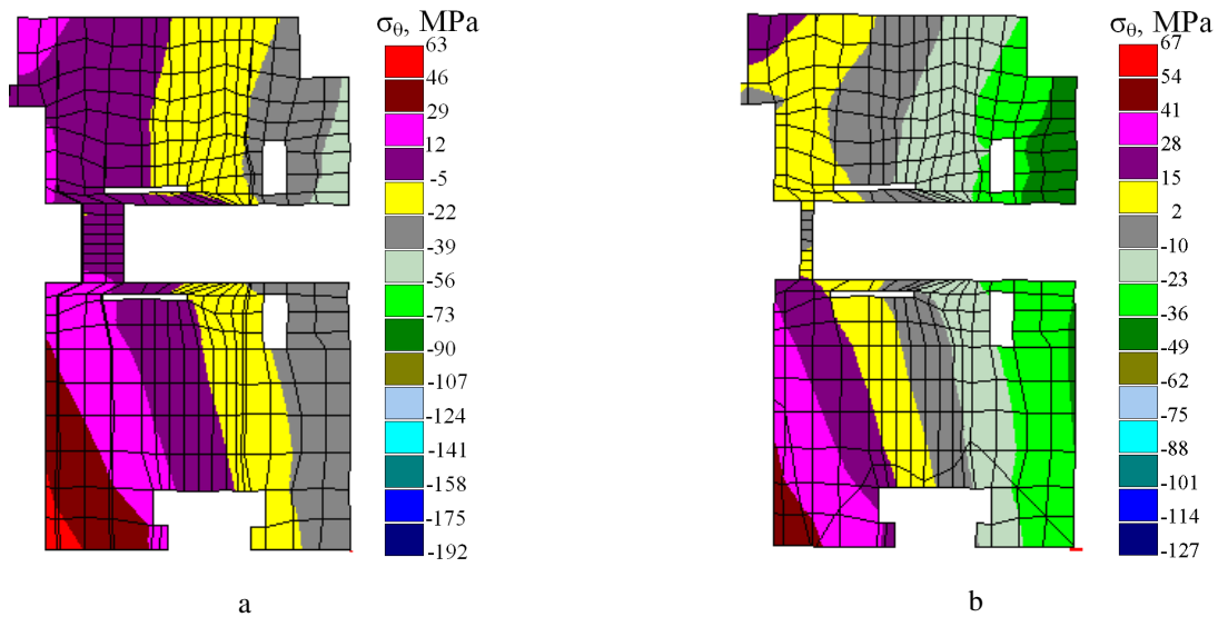
Fig. 9. Circumferential stresses in the rim and body in the middle cross-section of the diaphragm: a – in the elastic state; b – during creep
