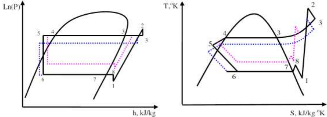
Figure 1. Thermodynamic cycle on diagrams temperature-entropy and pressure-enthalpy
