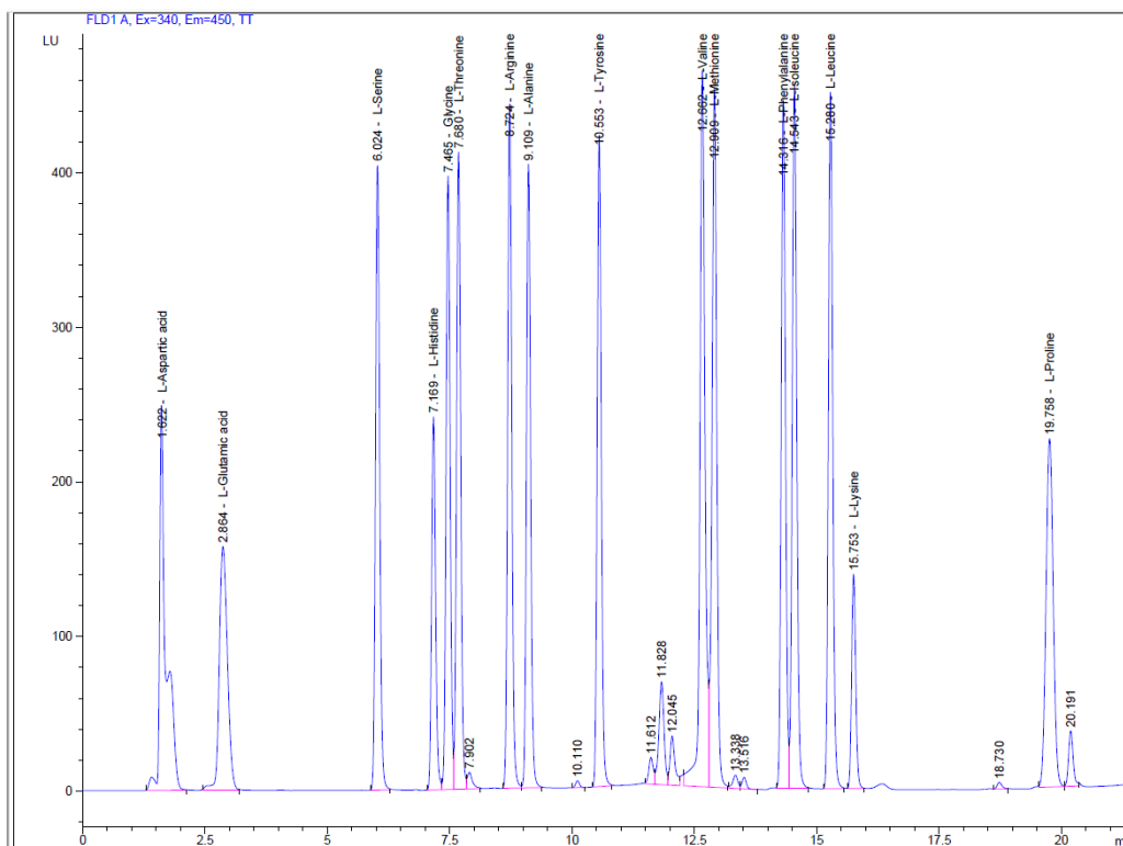
Fig. 1. Chromatogram definition of amino acids in the shubby Sophora roots
