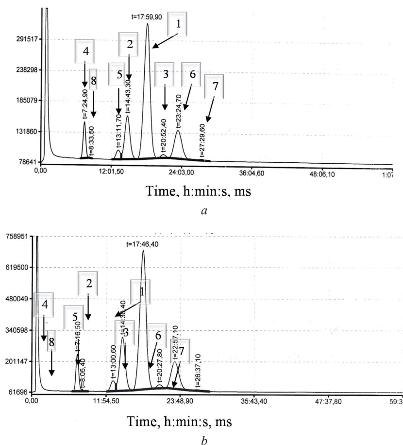
Fig. 2. The chromatogram of hemp oil methyl esters identified using the GC method: a – No. 1, 2019; b – No. 2, 2020; 1 – linoleic acid, 2 – oleic acid, 3 – linolenic acid, 4 – palmitic acid, 5 – stearic acid, 6 – linolenic acid, 7 – eicosenoic acid, 8 – palmitoleic acid
