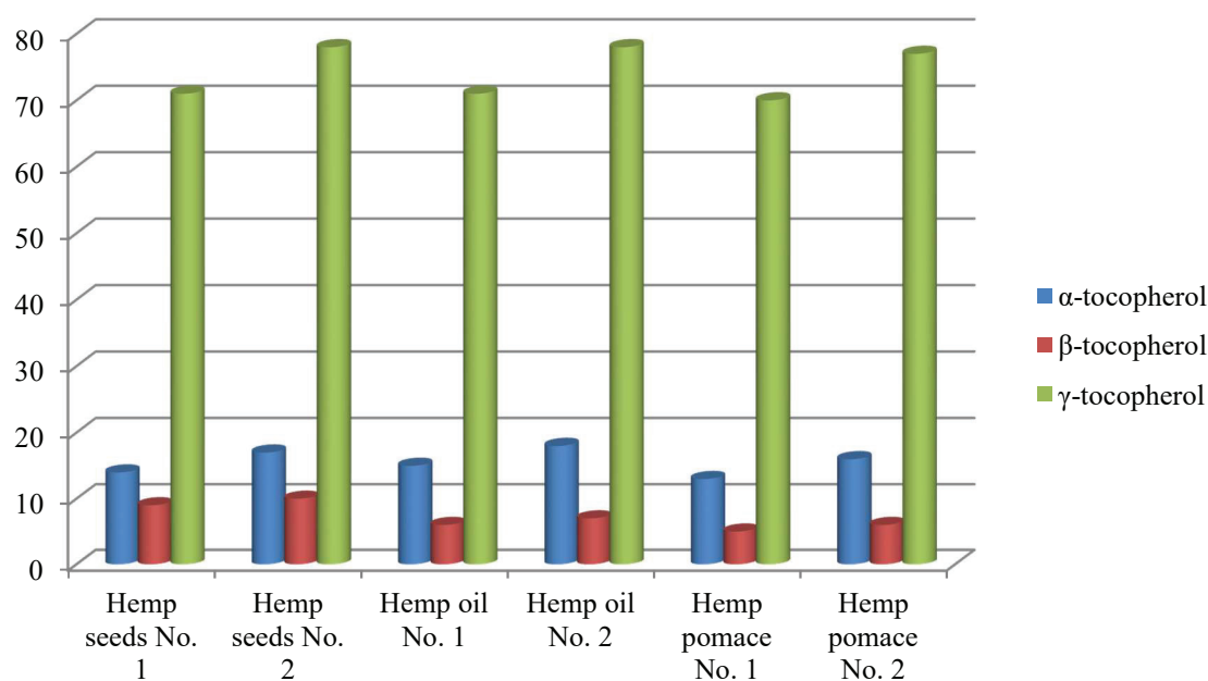
Fig. 3. The content of tocopherols in Cannabis sativa L. raw materials
