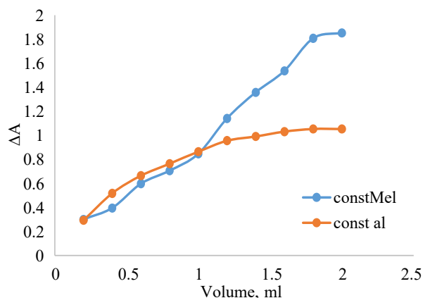
Fig. 7. Saturation curves: meldonium solution at a constant concentration of reagent (1.00 mL of 7.0 \times 10^{-3} M solution), alizarin solution at a constant concentration of meldonium (1.00 mL of 7.0 \times 10^{-3} M solution)
