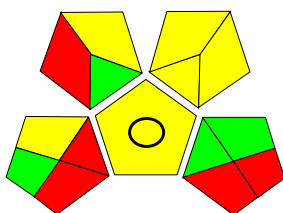
Fig. 9. Pictogram of analytical method using GAPI
