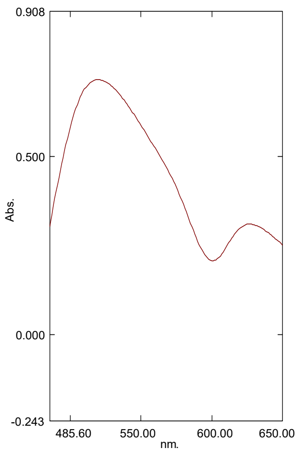
Fig. 1. Absorbance spectrum of the reaction product of meldonium ( C=6.25 \times 10^{-3} M) with 0.8 % solution of alizarine
