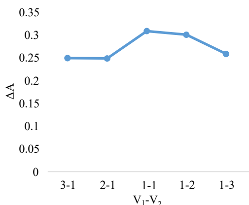
Fig. 6. Graph of the dependence of absorbance on the composition of the isomolar solution:
