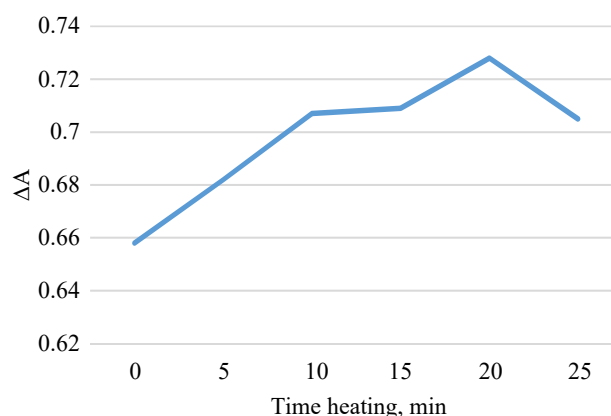
Fig. 3. The graph of dependence of the amount of absorbance of the reaction product of meldonium with alizarin depending on heating time
