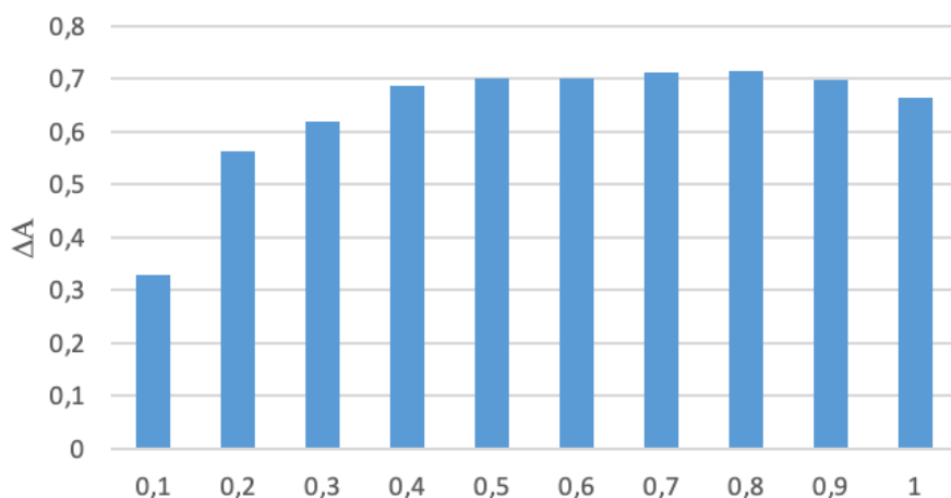
Fig. 2. The graph of dependence of the amount of absorbance depending on the concentration of the alizarine solution
