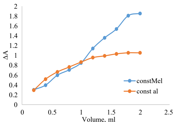
Fig. 7. Saturation curves: meldonium solution at a constant concentration of reagent (1.00 mL of 7.0×10 -3 M solution), alizarin solution at a constant concentration of meldonium (1.00 mL of 7.0×10 -3 M solution)
