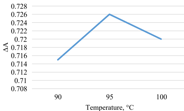
Fig. 4. The graph of dependence of the amount of absorbance of the reaction product of meldonium with alizarin depending on temperature
