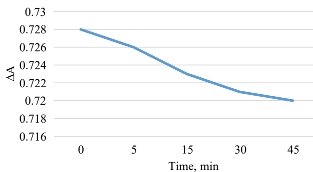
Fig. 5. Graph of the dependence of the absorbance of the reaction product of meldonium with alizarin depending on time
