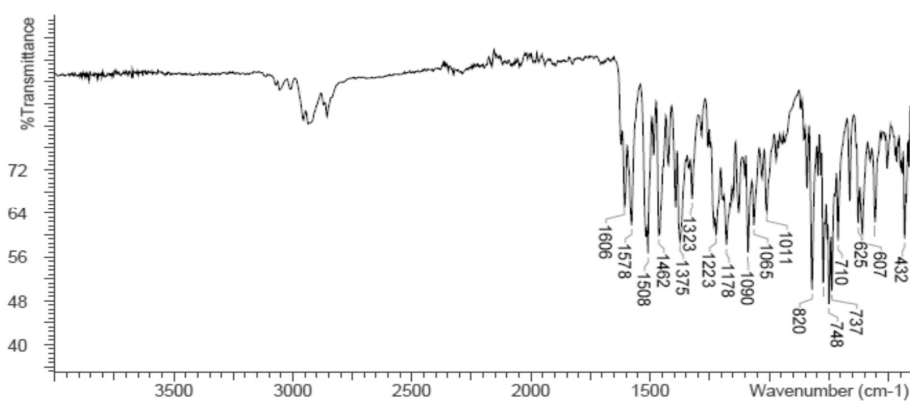
Fig. 5. IR spectrum of the investigated compound JWH-081
