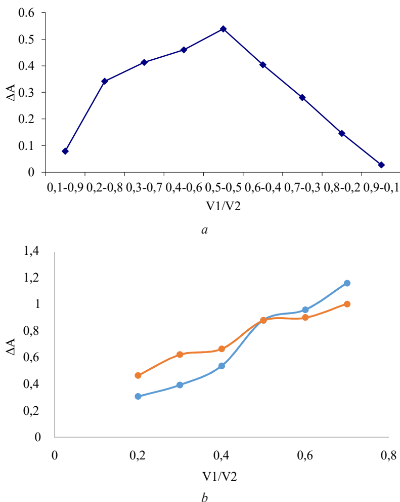
Fig. 7. Study of stoichiometric coefficients by the reaction with BPB: a – Ramipril: BPB complex continuous variation method at \lambda = 598 nm ( C_M = 2.35 \times 10^{-4} M); b – Molar ratio method of ramipril:BPB complex at \lambda = 598 nm ( C_{M \text{ BPB}} = 3.09 \times 10^{-4} M)
