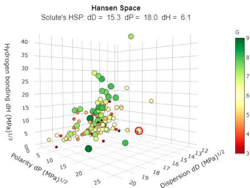
Fig. 6. Acetonitrile solvent sustainability level generated by the Hansen space green solvent selection tool
