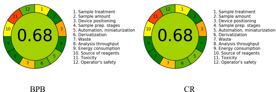
Fig. 9. Pictograms of analytical methods using AGREE tool
