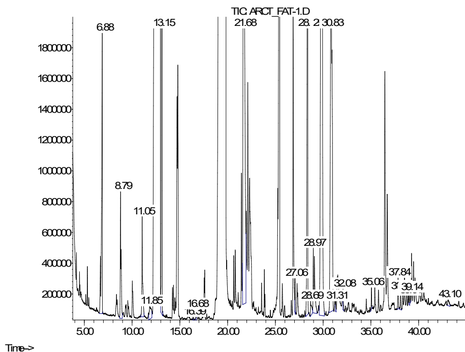
Fig. 2. Sample GC/MS chromatogram of organic, including fatty acids of the roots of A. lappa
