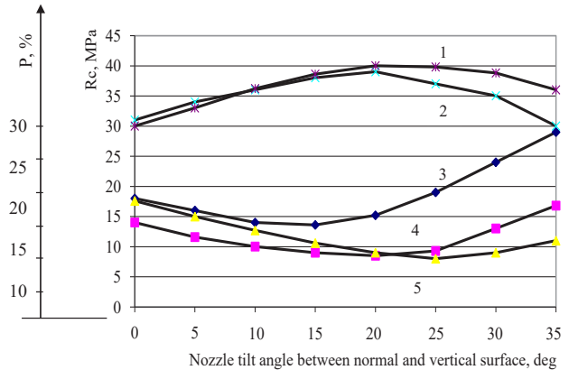
Fig. 4. Graph of dependences of the strength of the mixture and the amount of losses on the inclination angle of the nozzle to the vertical surface: 1, 2 – ultimate compressive strength, R_c , MPa; 3, 4, 5 – amount of losses, P , % (3 – layer strip thickness 30 \mu\text{m} , 1, 4 – mixture layer strip thickness 50 \mu\text{m} , 2, 5 – layer strip thickness 80 \mu\text{m} )
