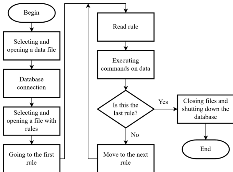
Fig. 6. The rule execution algorithm
