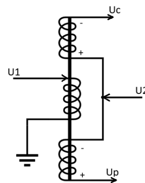
Fig. 2. Transformer circuit
