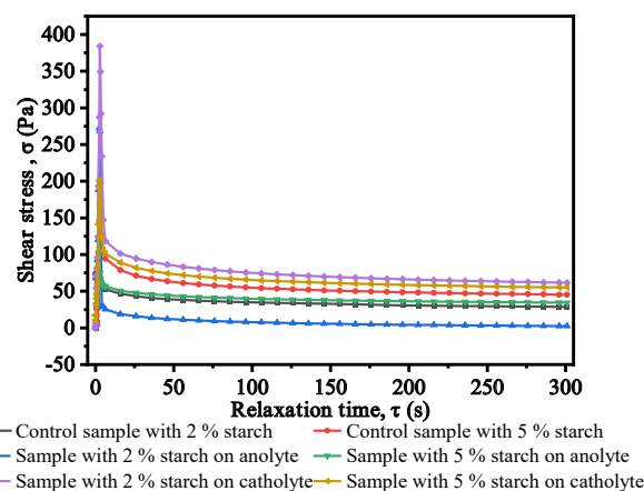
Fig. 1. The dependence of the change in the shear stress on the relaxation time of pate samples with different dosages of corn starch suspensions prepared on water with different RP indicators
