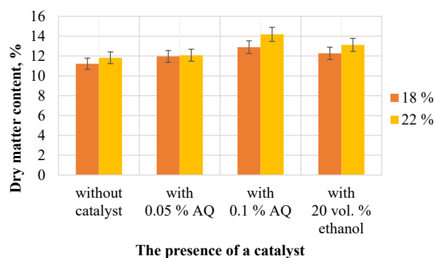
Fig. 3. The dependence of the content of dry matter in the black liquor on the consumption of active alkali and the use of catalysts during sodium boiling of Paulownia Clone in Vitro 112® wood for a duration of 150 min and a temperature of 170 °C
