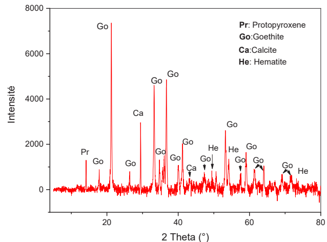
Fig. 2. X-ray diffraction spectrum of the initial sample
