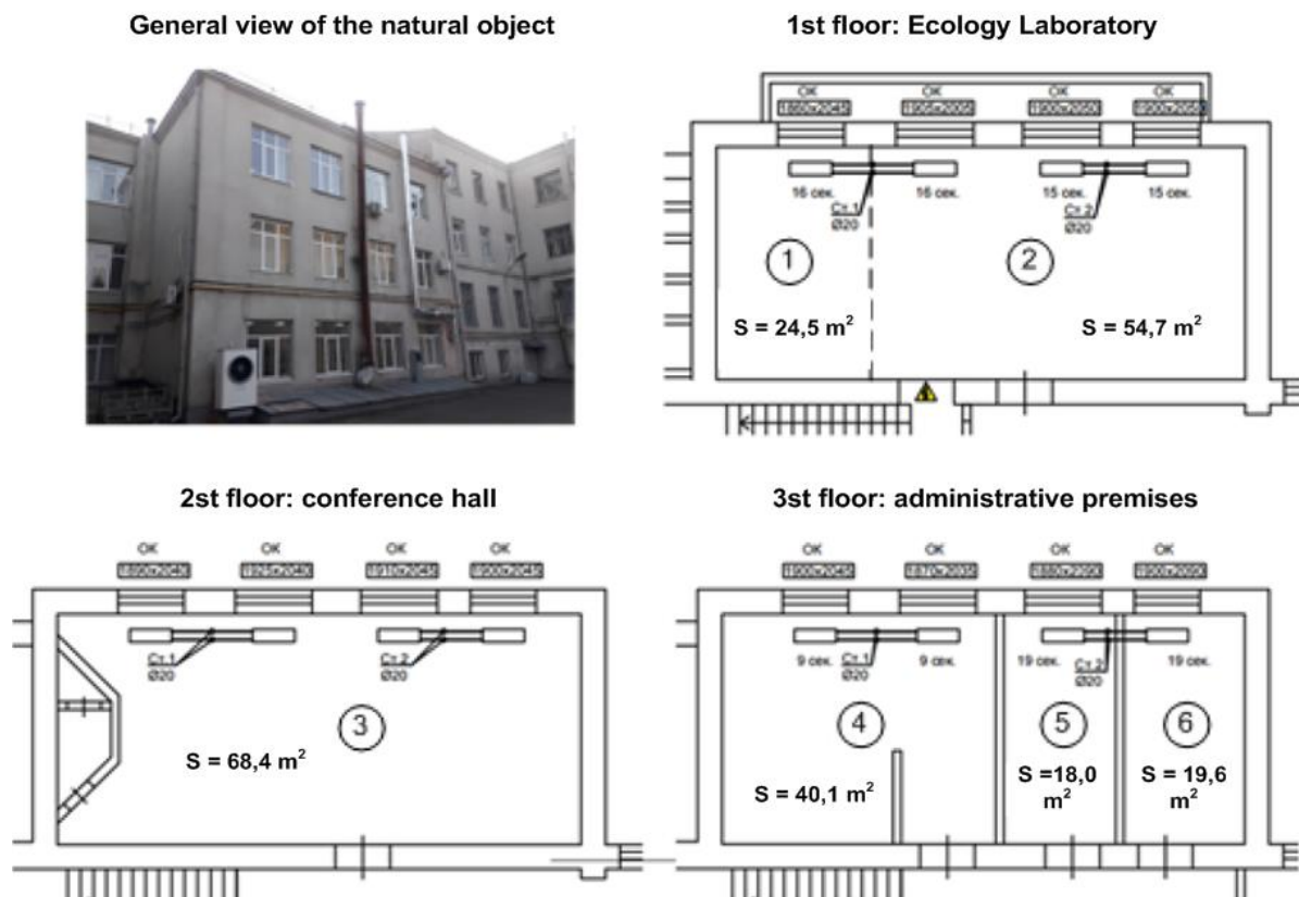
Fig. 1 – Natural object for research on the efficiency of heat consumption with total heated area 225.3 \text{ m}^2
